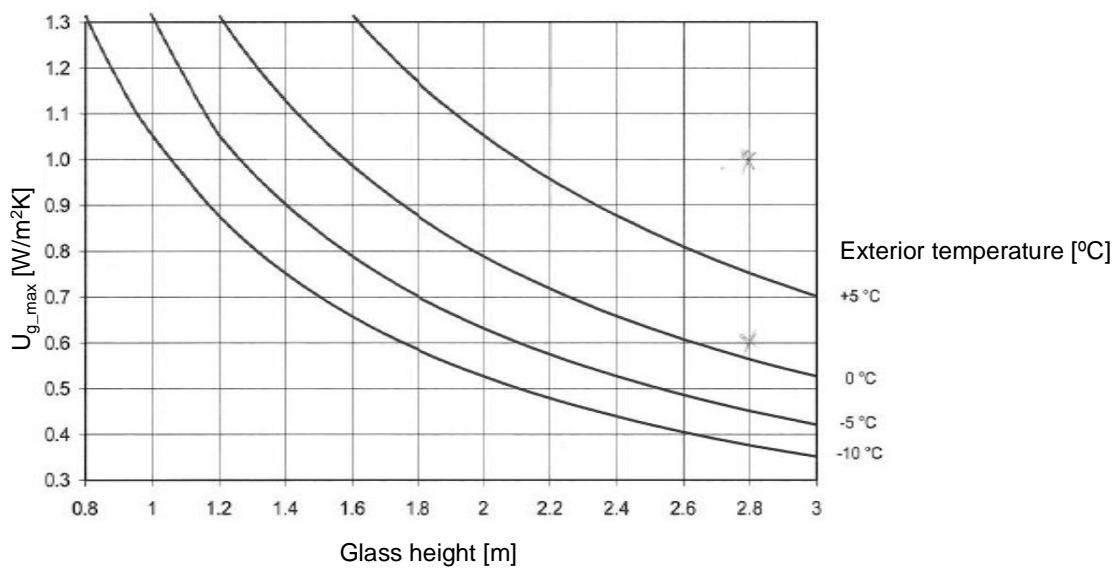
Figure 51: The influence of the window height and the outdoor temperature on the necessary U_g -value in order to avoid draught. From [16]
