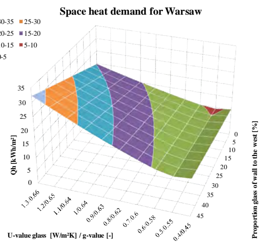
Figure 77. Effect of different window U-values (linked with the g-values) and different glass proportions on the given façade on the space heating demand in Warsaw. Fixed window size to every other orientation: N=1%, E=6%, S=54% and W=6%.
