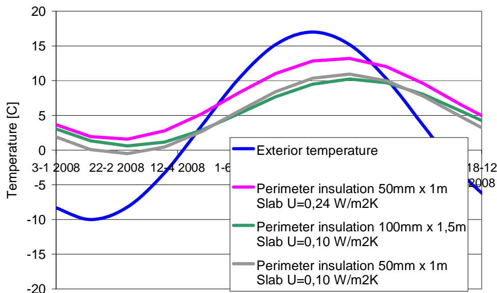
Figure 57: Monthly average exterior temperatures and resulting temperatures in the outermost corner of the foundation with different perimeter insulations. The conventional solution for the slab on ground ( U=0,24 \text{ W/m}^2\text{K} ) is compared with a very well insulated slab ( U=0,1 \text{ W/m}^2\text{K} ). The conventional perimeter insulation will result in insufficient frost protection of the very low energy house and more than doubling of the perimeter insulation is needed.
