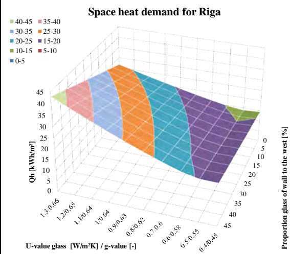
Figure 75. Effect of different window U-values (linked with the g-values) and different glass proportions on the given façade on the space heating demand in Riga. Fixed window size to every other orientation: N=1%, E=6%, S=54% and W=6%.
