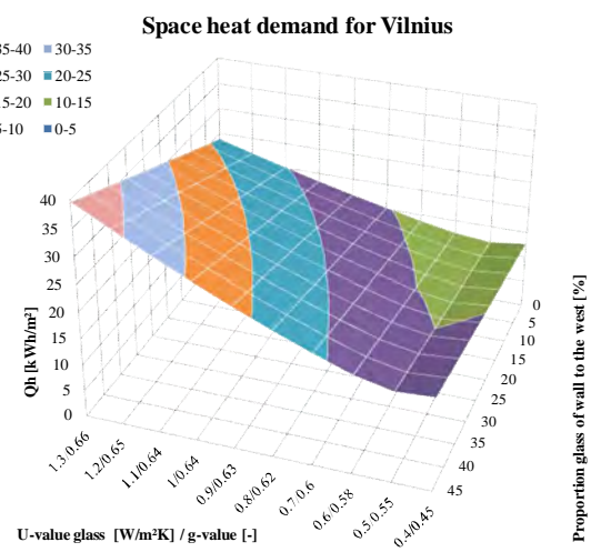
Figure 73. Effect of different window U-values (linked with the g-values) and different glass proportions on the given façade on the space heating demand in Vilnius. Fixed window size to every other orientation: N=1%, E=6%, S=54% and W=6%.
