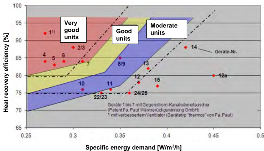
Figure 22. The heat recovery efficiency of different heat exchanger units as a function of power consumption [5].
