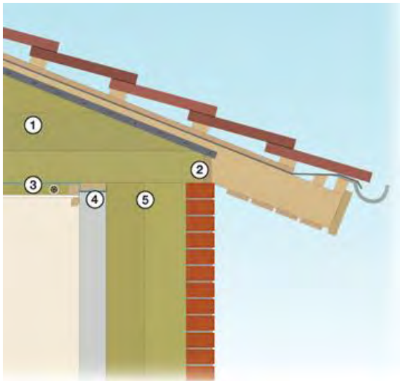
Figure 9. Roof/wall detail: 1. Insulation (2x145 + 120mm); 2. Wind barrier; 3. Insulation (45mm); 4. Airtight sealing; 5. Insulation (2x150mm) U\text{-value roof} = 0.08 U\text{-value wall} = 0.10 (Source: Rockwool.dk) 1
