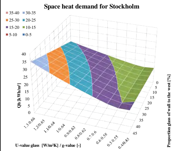
Figure 65. Effect of different window U-values (linked with the g-values) and different glass proportions on the given façade on the space heating demand in Stockholm. Fixed window size to every other orientation: N=1%, E=6%, S=54% and W=6%.
