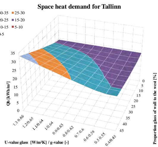
Figure 72 Effect of different window U-values (linked with the g-values) and different glass proportions on the given façade on the space heating demand in Tallinn. No windows to other directions..
