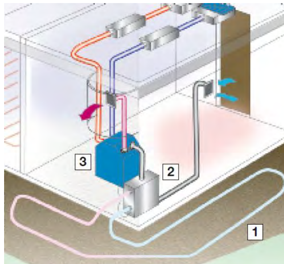
Figure 53. Earth-brine ground source heat exchanger: A brine filled ground loop (as geothermal probe or below the surface) is connected to a water/air heat exchanger which passes the energy of the brine to the ventilation air. (Source: Zehnder Comfosystems)
